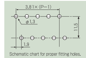
Schematic chart for proper fitting holes.
