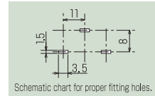
Schematic chart for proper fitting holes.
