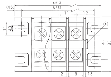
OK-020-□P-FC FINGER PROTECTING COVER (3~7Pole)
