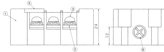
OK-020-□P-FC FINGER PROTECTING COVER (3~7Pole)
