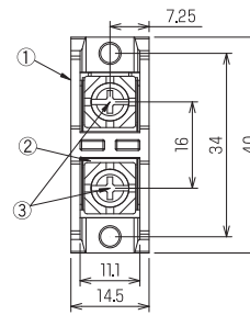
[DIN rail] OK-10R
