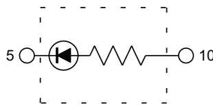
IND. LIGHT IN "C" SCHEMATIC
