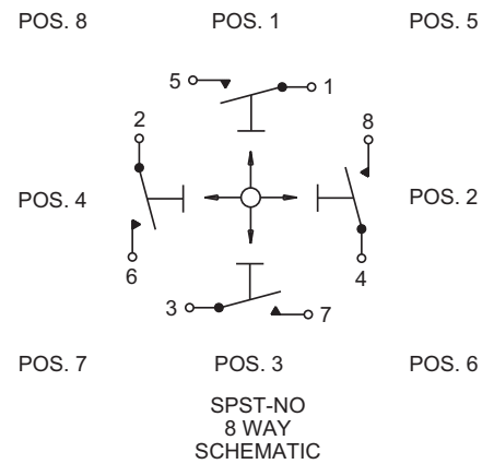
BUTTON POSITION/SWITCH ACTION (ALL MOMENTARY CONTACTS - ALL OTHER CONTACT SETS NOT SHOWN ARE OPEN)
