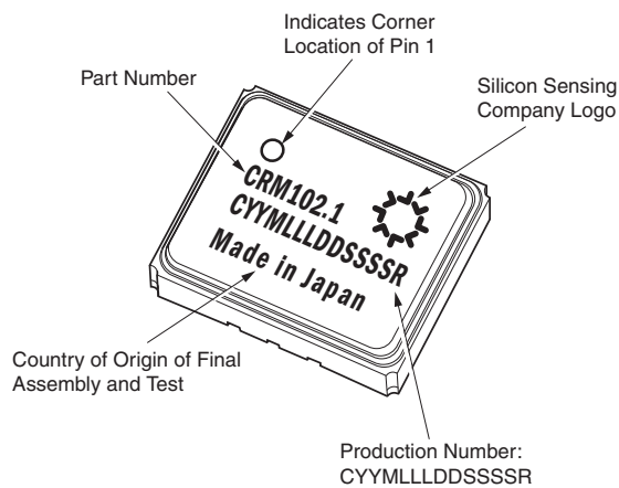
Figure 11.1 Part Marking
