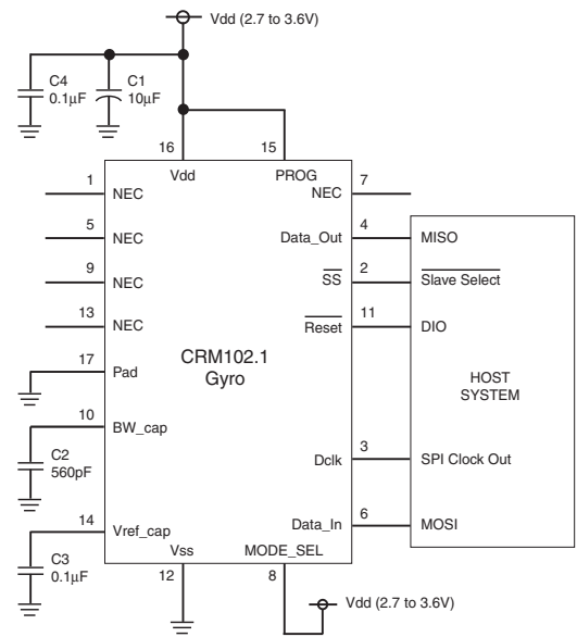
Figure 7.4 Peripheral Circuit - Digital Output (CRM102.1)
