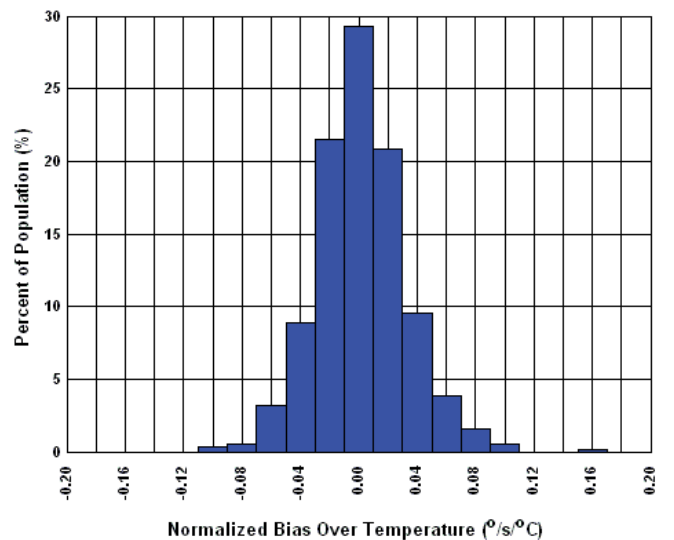
Figure 5.23 Normalized Digital Bias Over Temperature
