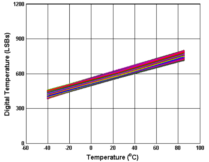
Figure 5.27 Digital Temperature Output (LSB) vs Temperature
