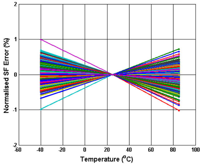
Figure 5.29 Digital Normalised Error (%) vs Temperature
