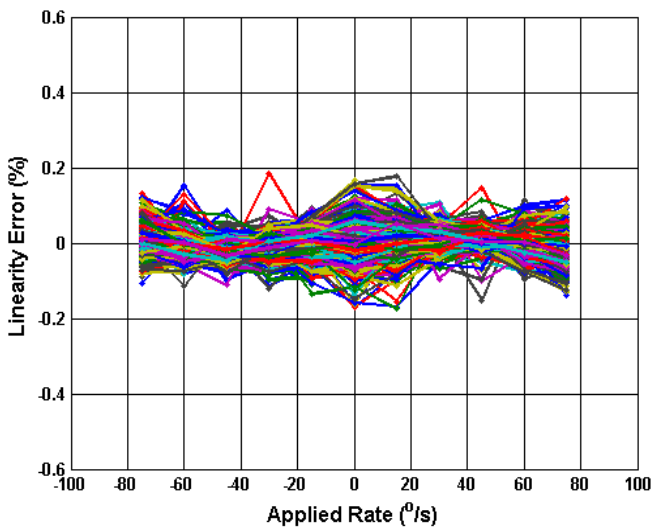
Figure 5.30 Digital NL Error (%) vs Applied Rate (-40°C)
