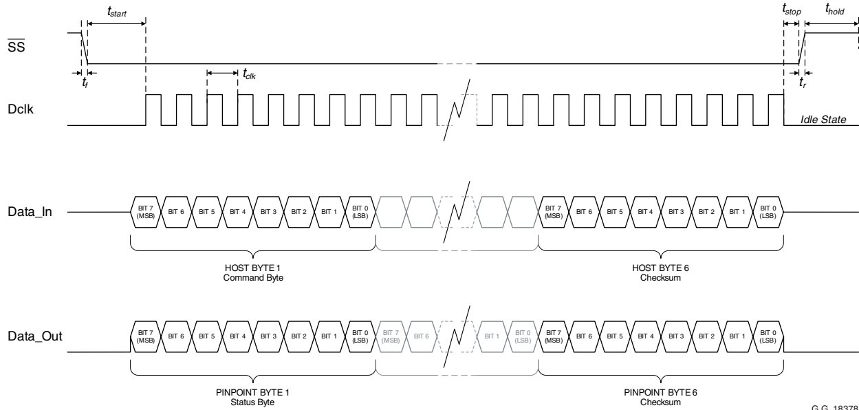
Figure 7.6 SPI ® Timing
