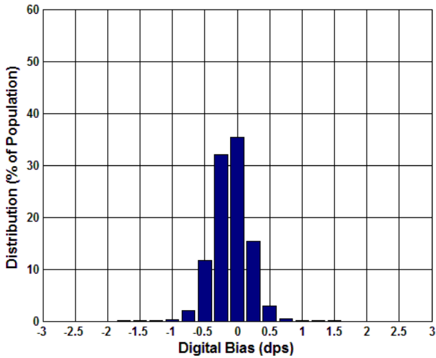
Figure 5.37 Digital Bias (dps) at 25°C
