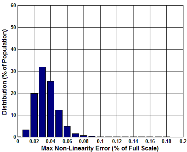
Figure 5.42 Digital Maximum Linear Error (%) at -40°C
