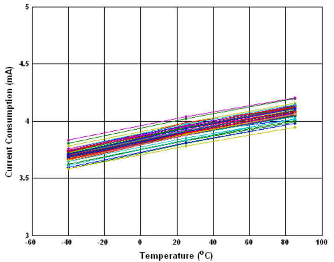
Figure 5.12 Current Consumption vs Temperature
