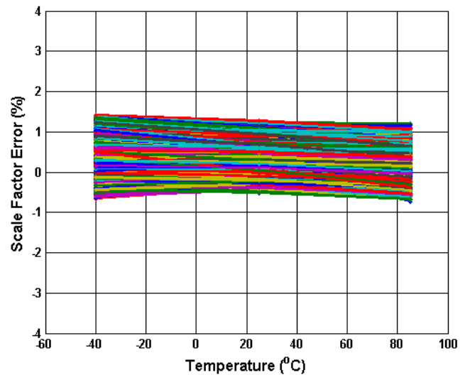
Figure 5.28 Digital Scale Factor Error (%) vs Temperature
