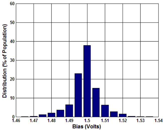
Figure 5.13 Analogue Bias (Volts) Over Temperature
