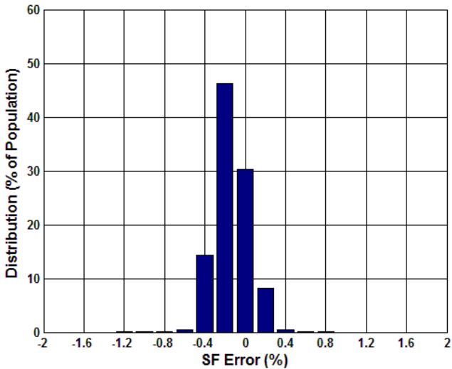
Figure 5.41 Digital Normalised SF Error (%) over Temperature
