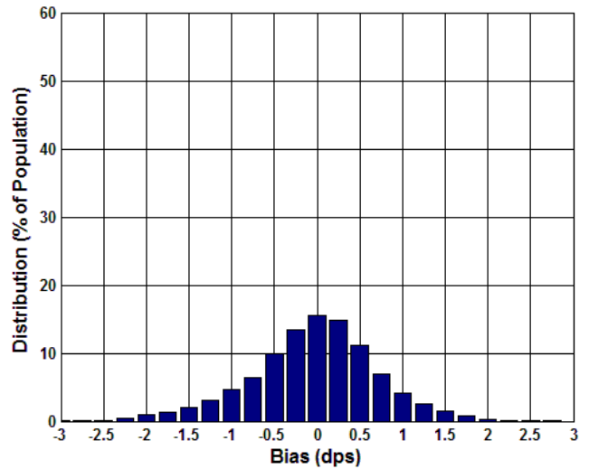
Figure 5.15 Analogue Normalised Bias Distribution (dps) Over Temperature
