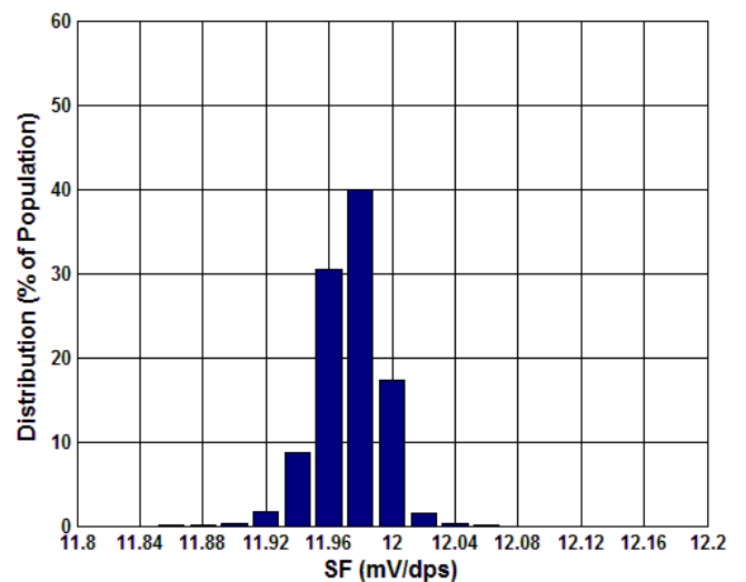
Figure 5.20 Analogue SF at 25°C
