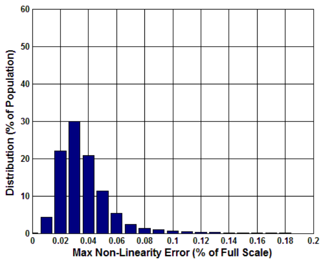
Figure 5.44 Digital Maximum Linear Error (%) at 85°C
