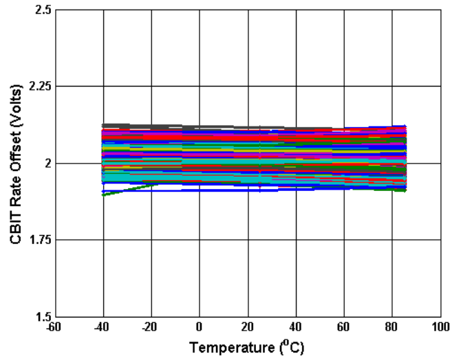
Figure 5.11 Analogue CBIT Offset (Volts) vs Temperature
