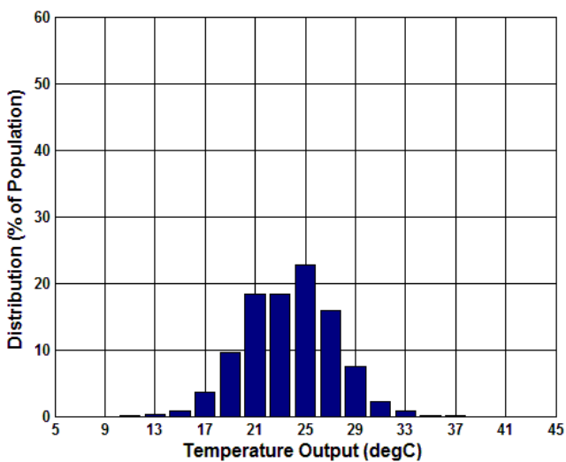
Figure 5.46 Temperature Output (°C) at 25°C
