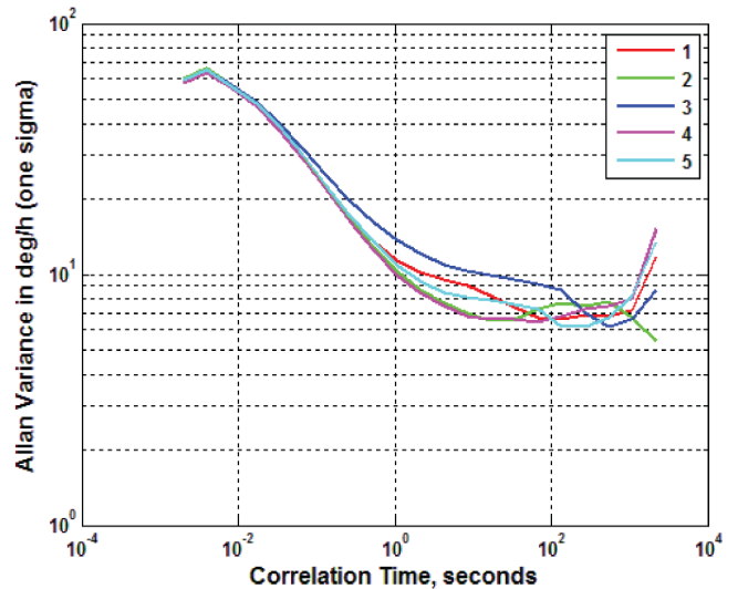
Figure 5.52 Allan Variance of CRM100s 75°/s 25Hz
