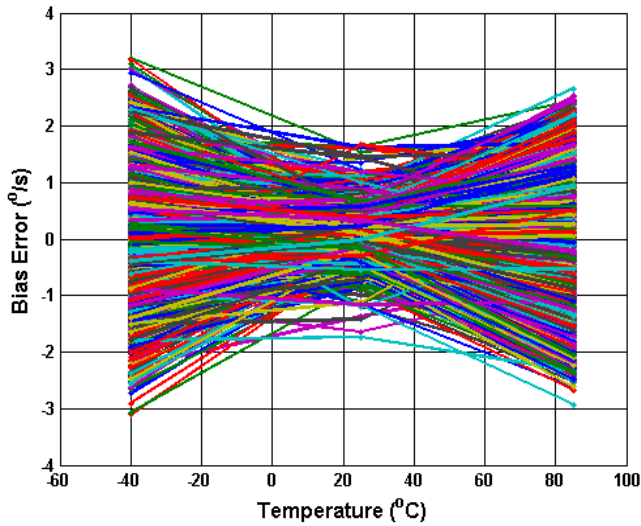
Figure 5.25 Digital Bias Error (dps) vs Temperature
