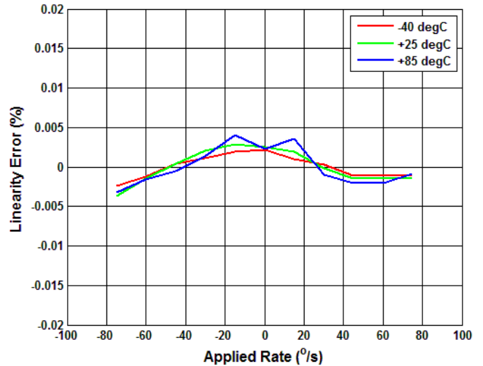
Figure 5.7 Analogue Ave NL Error (%) vs Applied Rate
