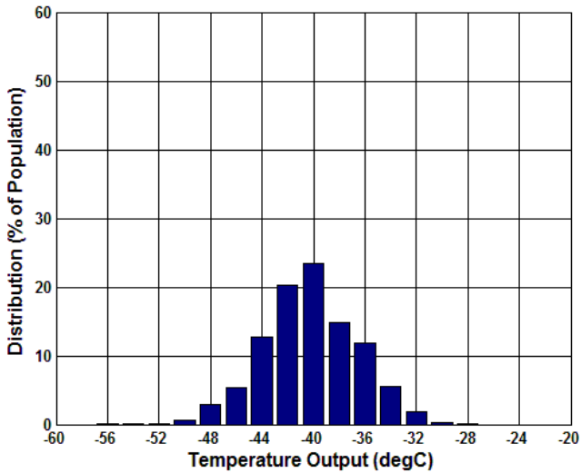
Figure 5.45 Temperature Output (°C) at -40°C
