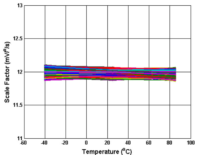
Figure 5.4 Analogue Scale Factor vs Temperature
