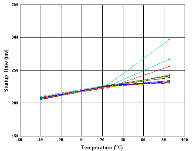
Figure 5.48 Startup Time vs Temperature (Vdd = 2.7V)
