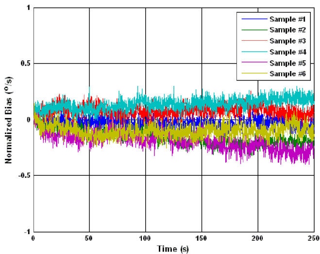
Figure 5.50 Normalised Bias Drift after Switch-On
