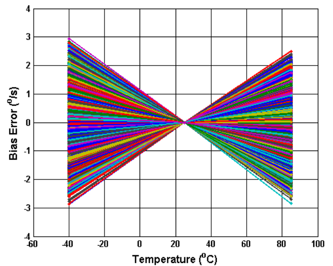
Figure 5.3 Analogue Normalised Bias Error (dps) vs Temperature
