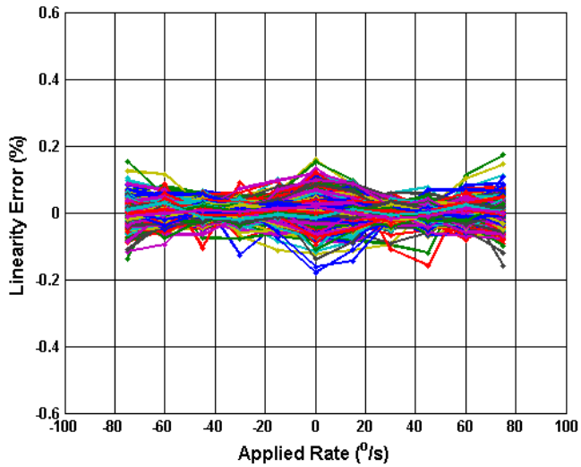
Figure 5.9 Analogue NL Error (%) vs Applied Rate (25°C)
