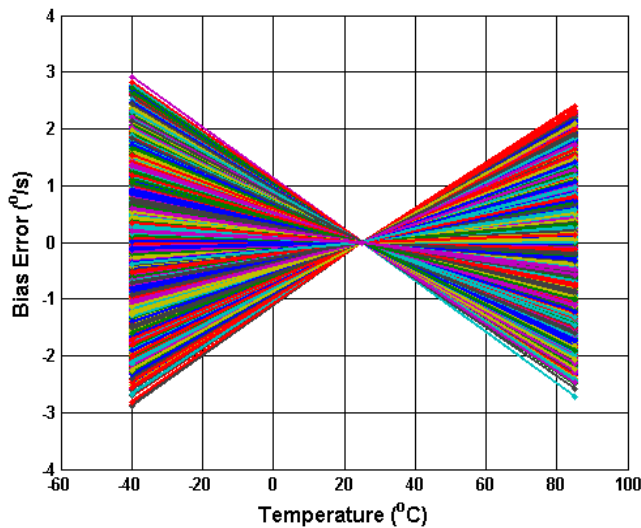
Figure 5.26 Digital Normalised Bias Error (dps) vs Temperature
