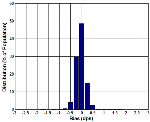
Figure 5.17 Analogue Bias (dps) at 25°C
