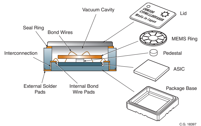
Figure 13.1 CRM100 Main Components
