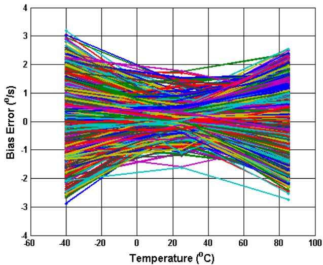
Figure 5.2 Analogue Bias Error (dsp) vs Temperature
