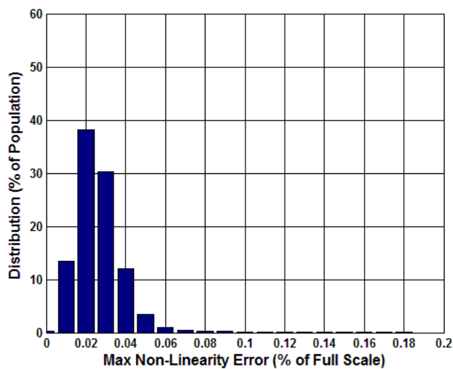
Figure 5.22 Analogue Maximum Linear Error (%) at -40°C
