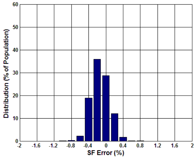
Figure 5.21 Analogue Normalised SF Error (%) Over Temperature
