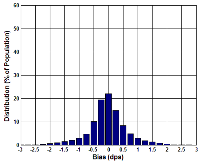
Figure 5.36 Digital Bias Distribution (dps) over Temperature
