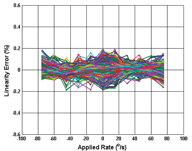
Figure 5.32 Digital NL Error (%) vs Applied Rate (85°C)
