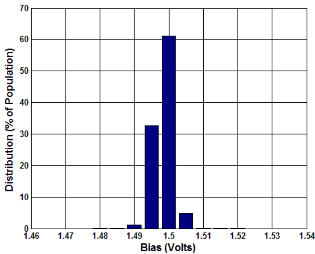
Figure 5.14 Analogue Bias at 25°C
