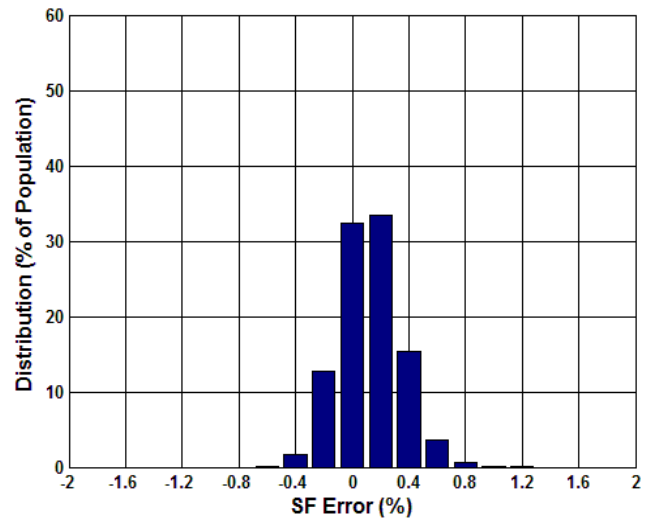
Figure 5.40 Digital SF Error (%) at 25°C
