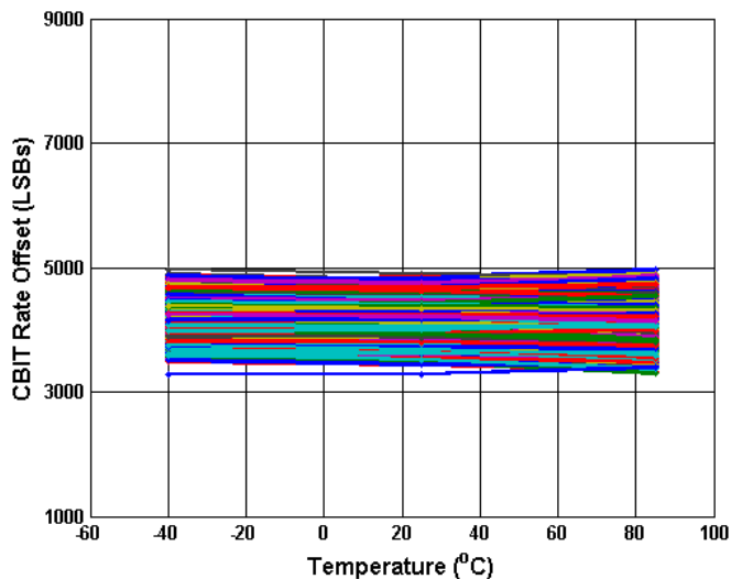
Figure 5.34 Digital CBIT (LSB) vs Temperature
