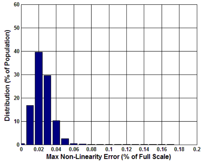
Figure 5.23 Analogue Maximum Linear Error (%) at 25°C
