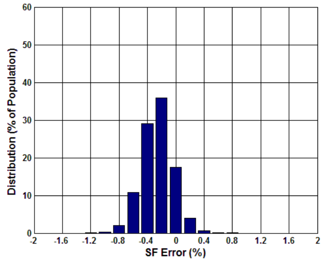
Figure 5.19 Analogue SF Error (%) Over Temperature
