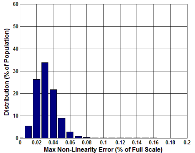
Figure 5.43 Digital Maximum Linear Error (%) at 25°C
