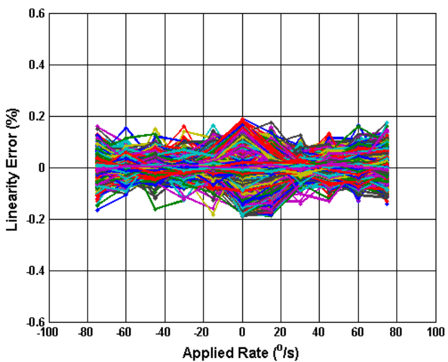
Figure 5.10 Analogue NL Error (%) vs Applied Rate (85°C)
