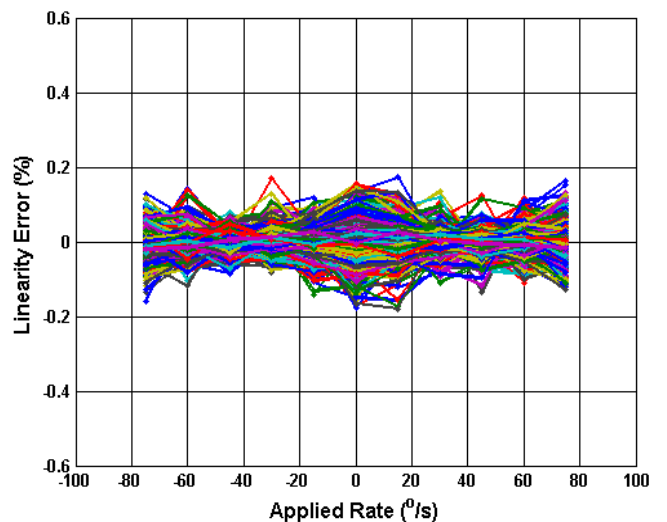
Figure 5.8 Analogue NL Error (%) vs Applied Rate (-40°C)
