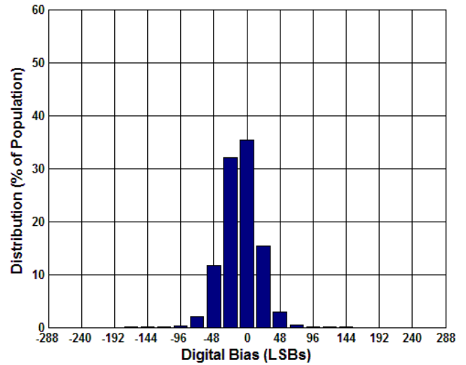
Figure 5.35 Digital Bias (LSB) at 25°C
