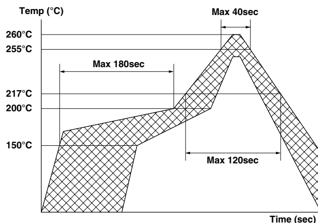
Figure 10.1 Recommended Reflow Solder Profile
