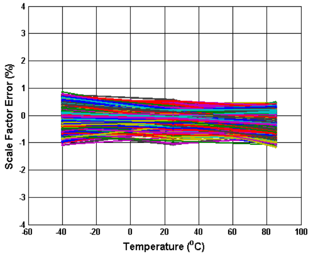
Figure 5.5 Analogue Scale Factor Error (%) vs Temperature
