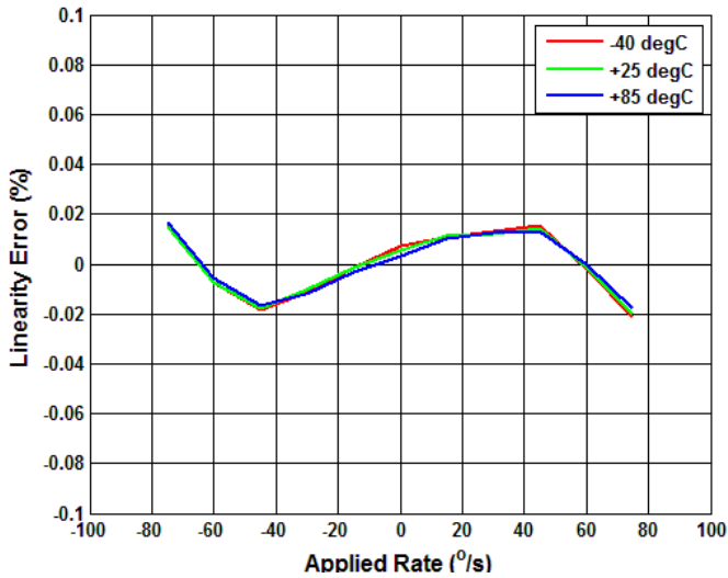
Figure 5.33 Digital Ave Error (%) vs Applied Rate
