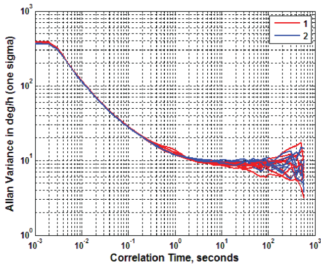
Figure 5.53 Allan Variance of CRM100s 900°/s 150Hz
