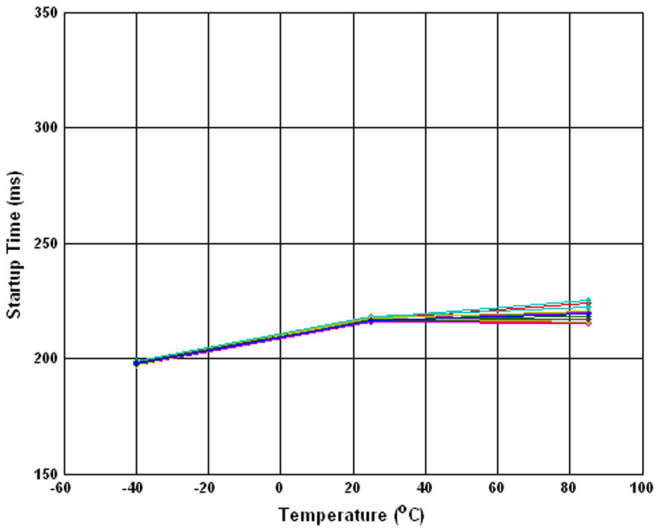
Figure 5.49 Startup Time vs Temperature (Vdd = 3.6V)
