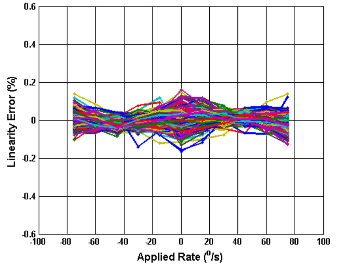
Figure 5.31 Digital NL Error (%) vs Applied Rate (25°C)
