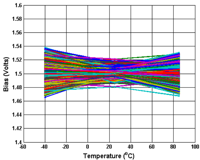
Figure 5.1 Analogue Bias (Volts) vs Temperature
