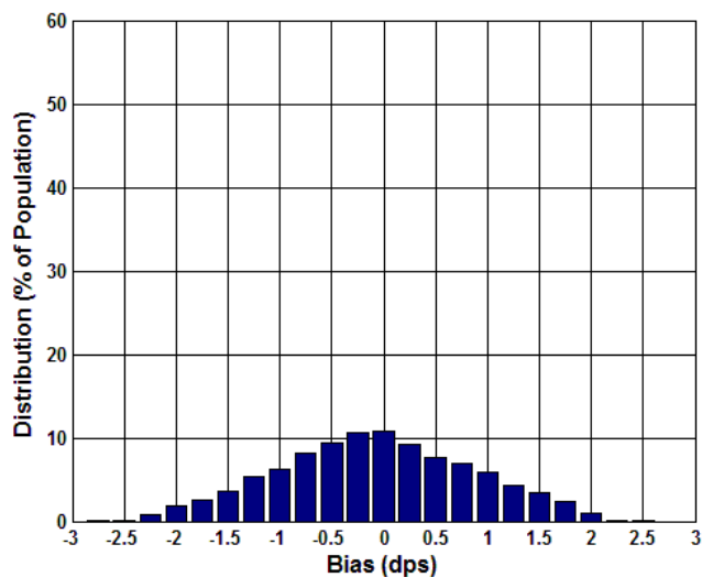
Figure 5.18 Analogue Bias (dps) at 85°C
