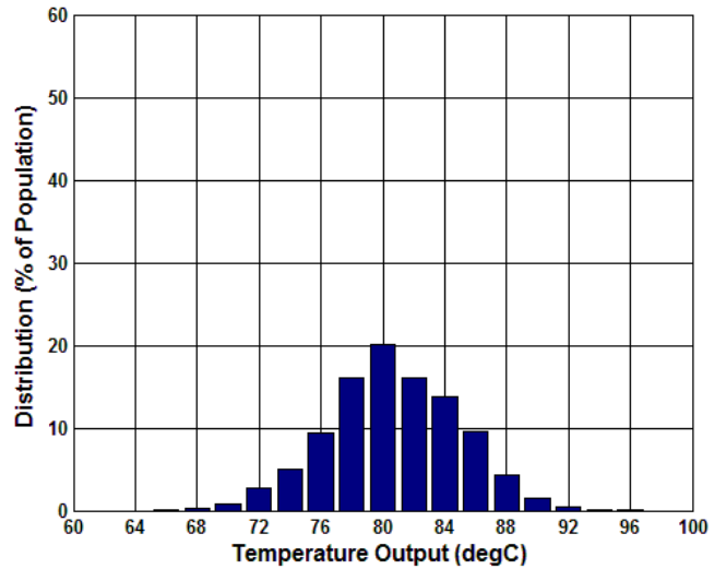
Figure 5.47 Temperature Output (°C) at 85°C
