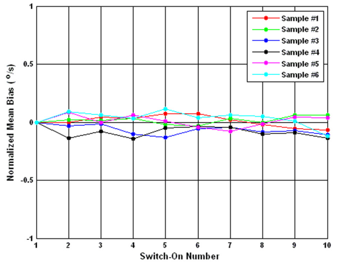
Figure 5.51 Switch-On Repeatability of Normalised Mean Bias
