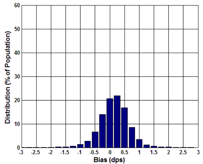
Figure 5.16 Analogue Bias (dps) at -40°C
