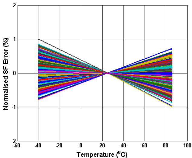
Figure 5.6 Analogue Normalised Scale Factor Error (%) vs Temperature
