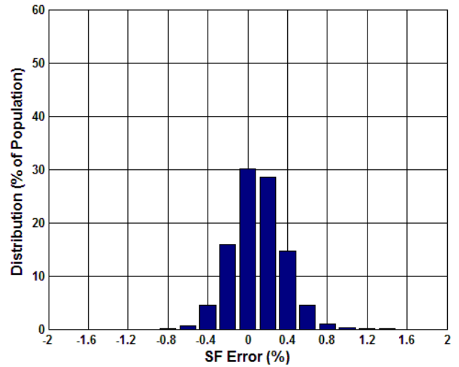
Figure 5.39 Digital SF Error (%) over Temperature
