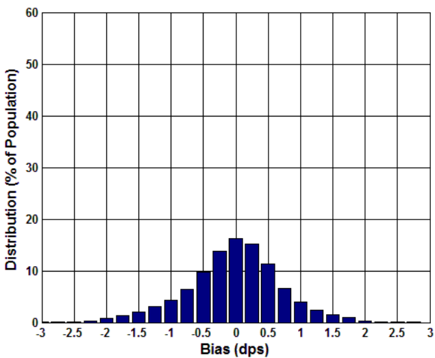
Figure 5.38 Digital Normalised Bias Distribution (dps) over Temperature
