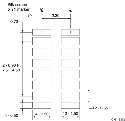
Figure 7.2 Recommended Pad Layout (CRM200)
