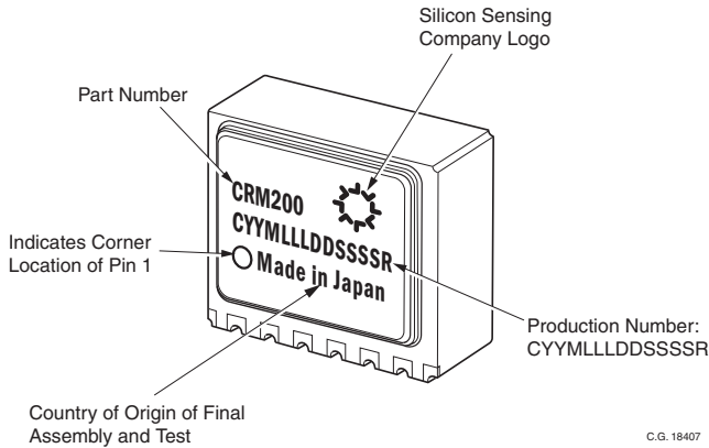
Figure 11.1 Part Marking
