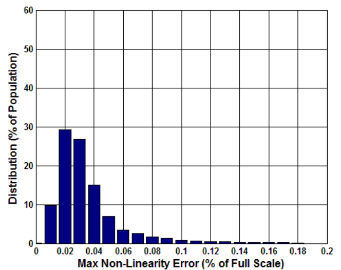
Figure 5.24 Analogue Maximum Linear Error (%) at 85°C
